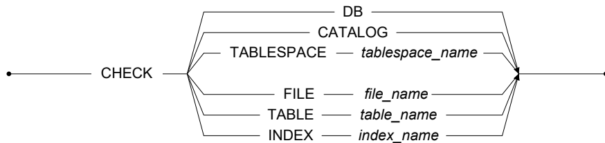
Figure 3-38 CHECK syntax
