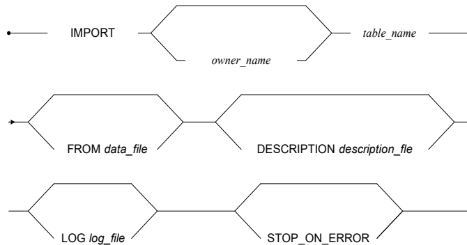
Figure 6-8 IMPORT syntax
