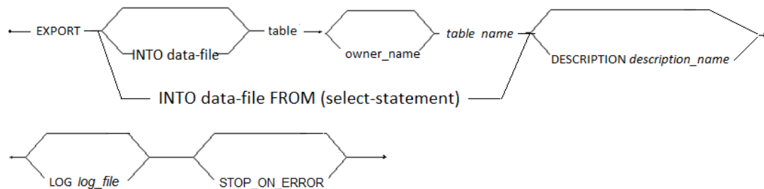
Figure 6-7 EXPORT syntax
