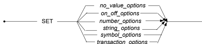
Figure 3-144 SET CONNECTION OPTIONS syntax
