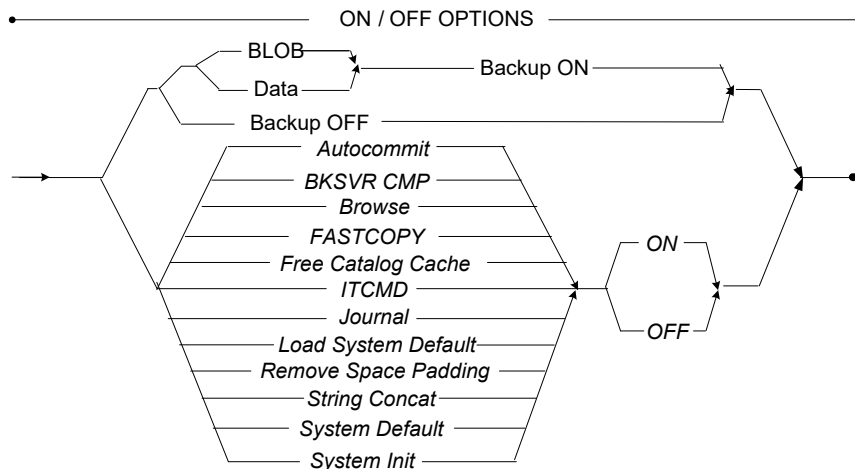
Figure 3-146 ON/OFF Options syntax
