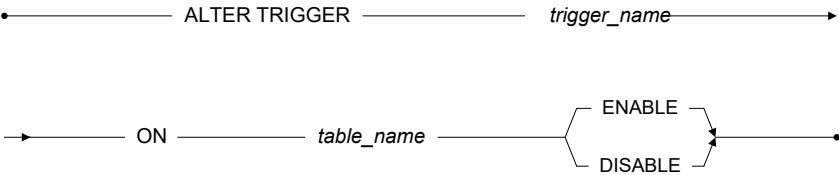
Figure 3-32 ALTER TRIGGER ENABLE syntax
