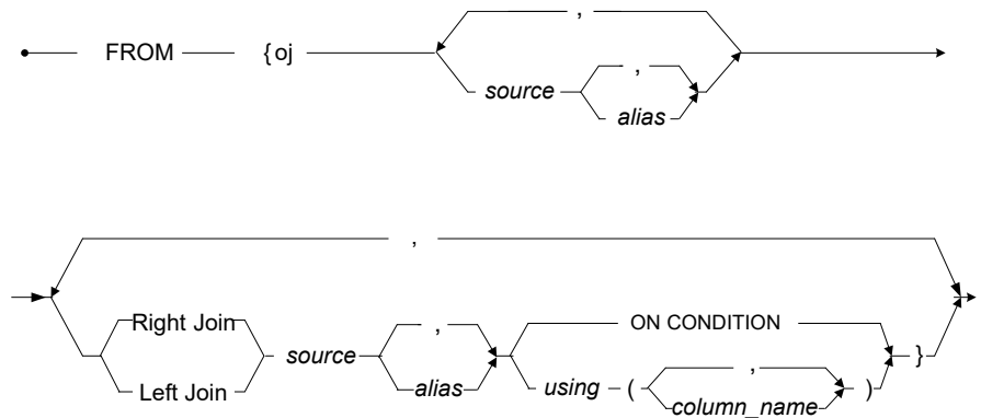
Figure 3-132 ODBC Outer-Join Syntax
