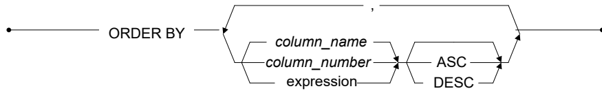
Figure 3-138 ORDER BY Clause syntax
