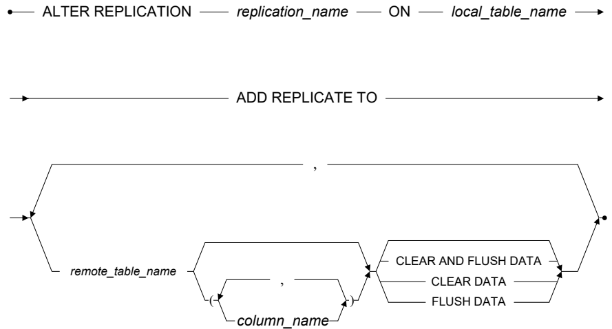
Figure 3-9 ALTER REPLICATION ADD REPLICATE syntax
