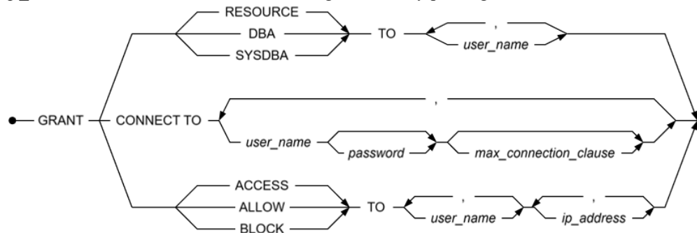
Figure 3-95 GRANT (Security Privileges) syntax
