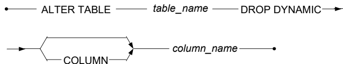
Figure 3-16 ALTER TABLE DROP DYNAMIC COLUMN syntax
