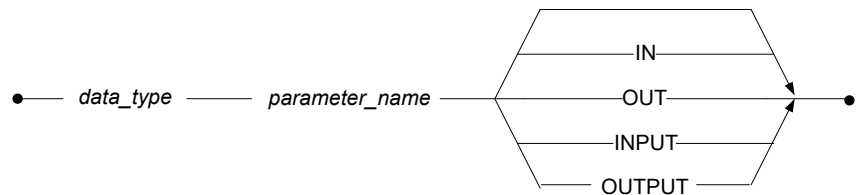
Figure 3-53 CREATE PROCEDURE: procedure_parameter syntax
