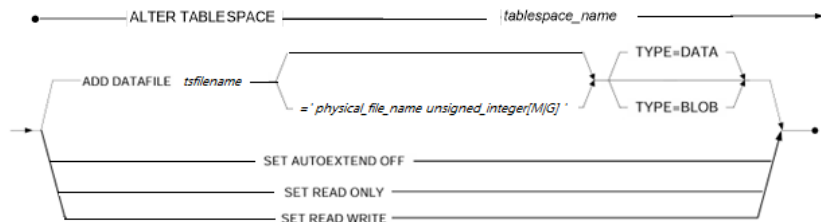
Figure 3-30 ALTER TABLESPACE syntax
