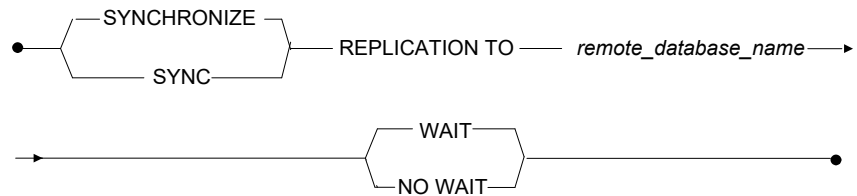
Figure 3-156 SYNCHRONIZE SCHEDULE syntax
