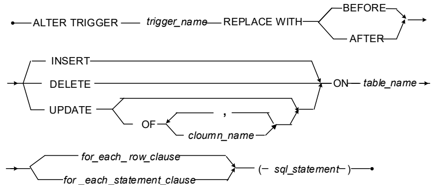
Figure 3-33 ALTER TRIGGER REPLACE syntax
