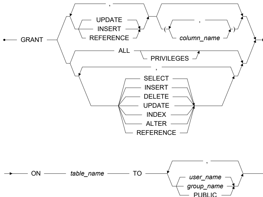
Figure 3-94 GRANT (Object Privileges) syntax
