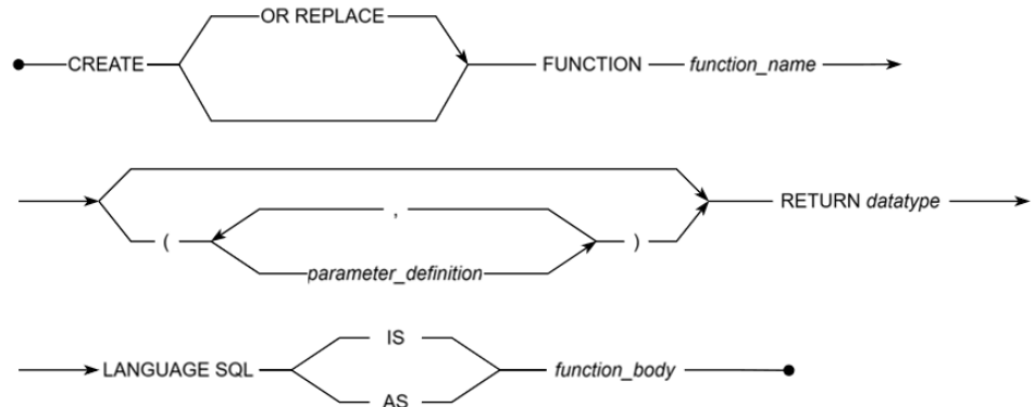
Figure 3-45 CREATE FUNCTION syntax
