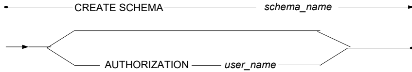
Figure 3-59 CREATE SCHEMA syntax
