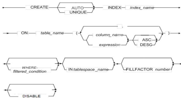
Figure 3-50 CREATE INDEX syntax
