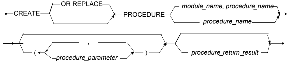
Figure 3-52 CREATE PROCEDURE syntax
