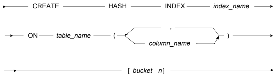
Figure 3-49 CREATE HASH INDEX syntax
