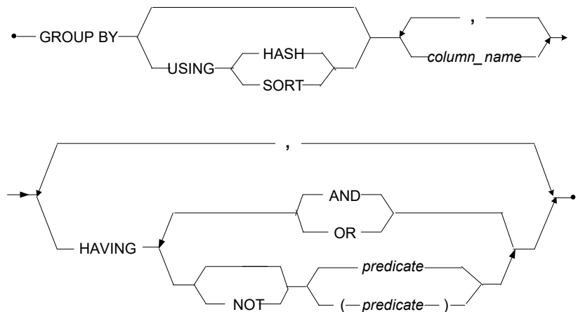
Figure 3-136 GROUP BY Clause syntax
