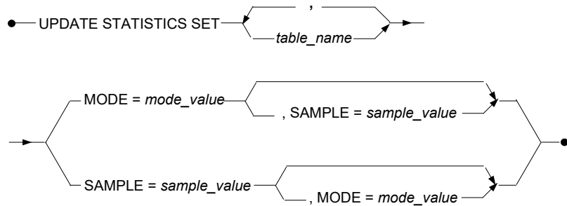
Figure 3-163 UPDATE STATISTICS SET syntax
