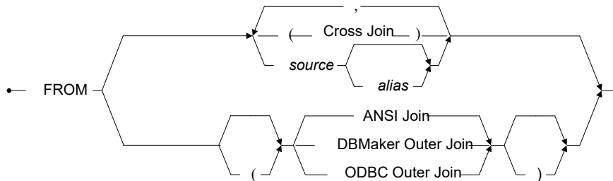
Figure 3-117 FROM Clause syntax
