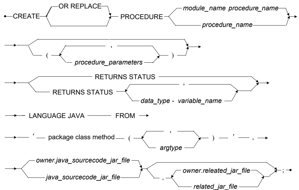
Figure 3-55 CREATE JavaSP syntax
