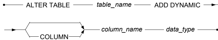
Figure 3-14 ALTER TABLE ADD DYNAMIC COLUMN syntax
