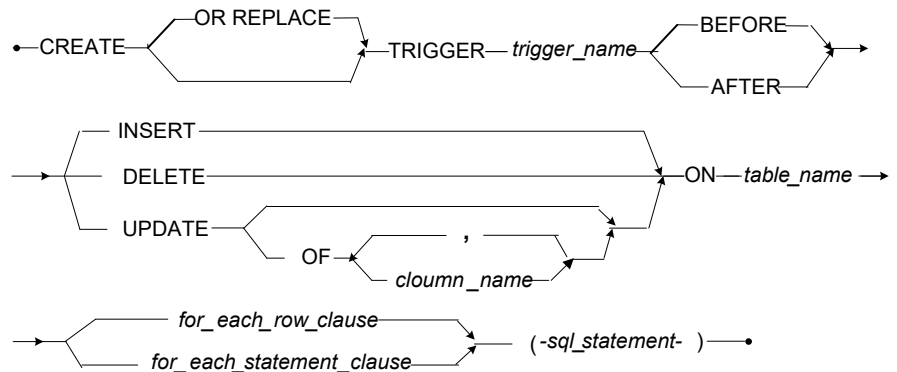
Figure 3-69 CREATE TRIGGER syntax
