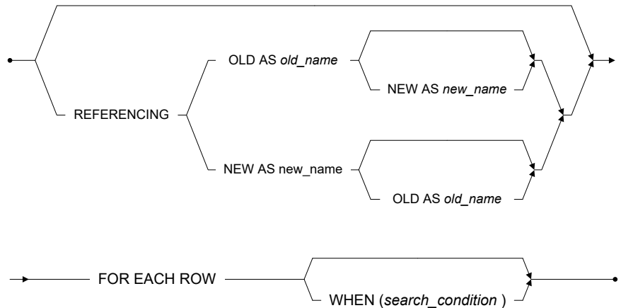
Figure 3-34 For Each Row Clause syntax
