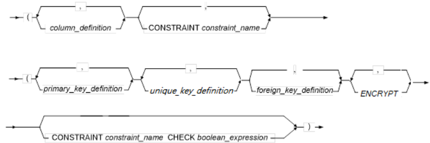
Figure 3-58 CREATE TABLE: table_column_definition syntax
