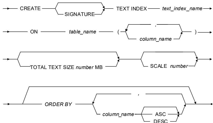
Figure 3-67 CREATE SIGNATURE TEXT INDEX syntax
