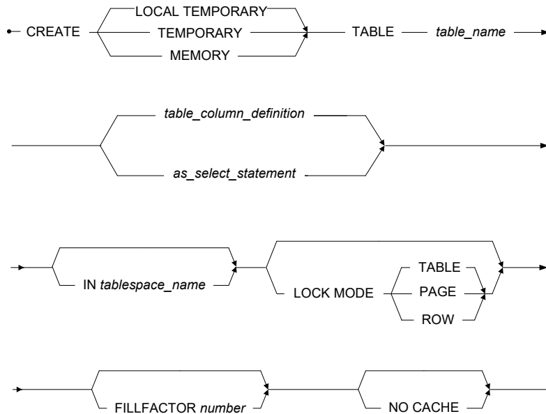
Figure 3-61 CREATE TABLE syntax
