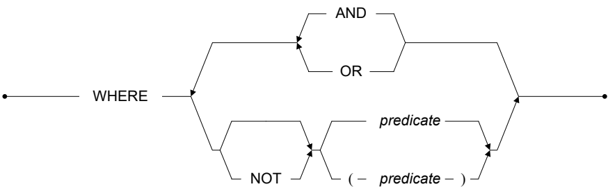
Figure 3-124 WHERE Clause syntax
