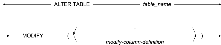
Figure 3-20 ALTER TABLE MODIFY COLUMN syntax
