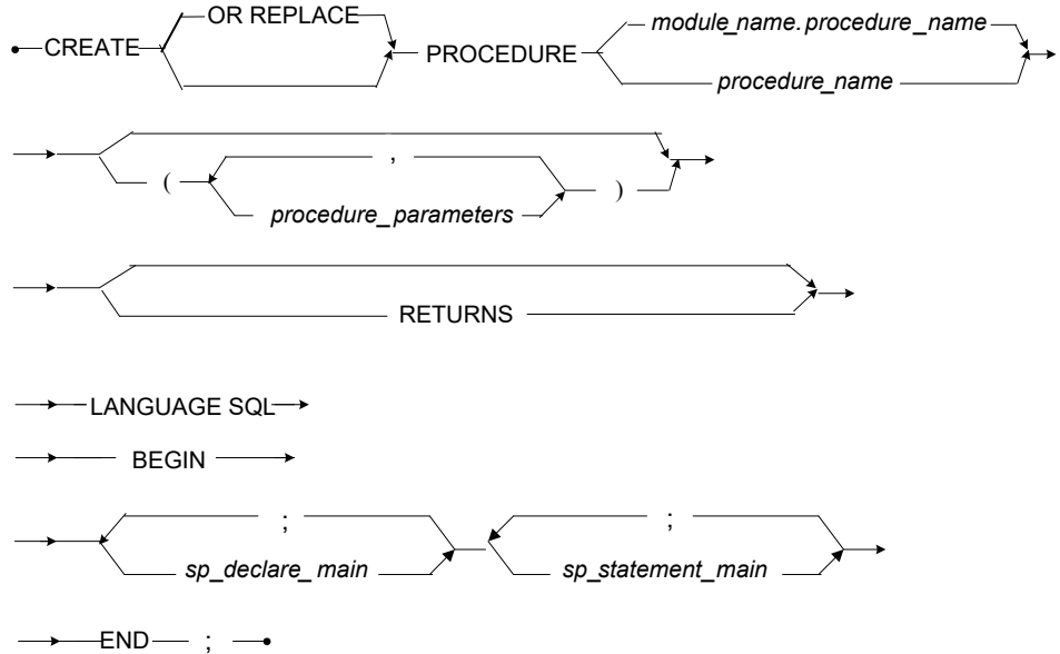
Figure 3-56 CREATE SQL SP syntax
