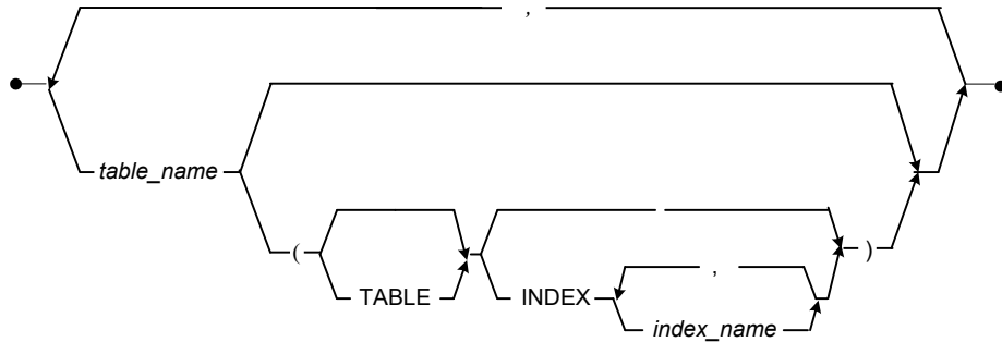
Figure 3-159 UNLOAD STATISTICS Object List syntax
