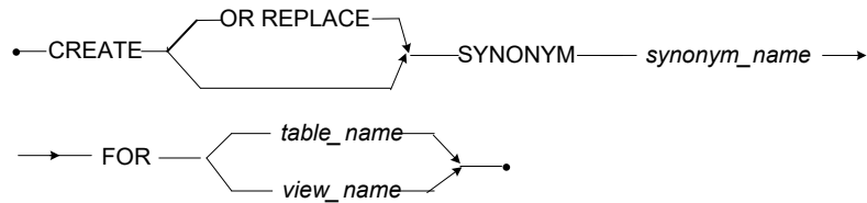
Figure 3-60 CREATE SYNONYM syntax
