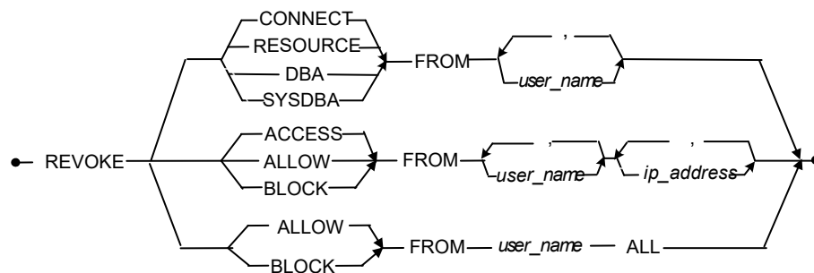
Figure 3-111 REVOKE (Security Privileges) syntax
