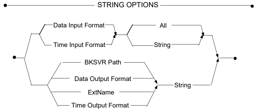
Figure 3-149 String Options syntax
