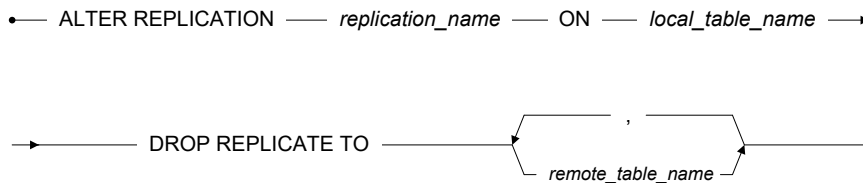
Figure 3-10 ALTER/DROP REPLICATION syntax
