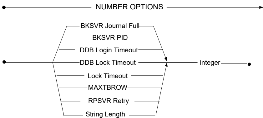
Figure 3-148 Number Options syntax
