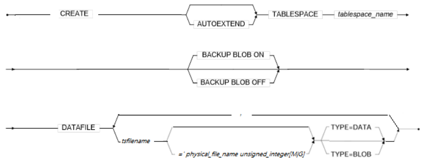
Figure 3-66 CREATE TABLESPACE syntax
