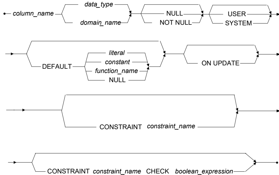
Figure 3-63 Column Definitions syntax
