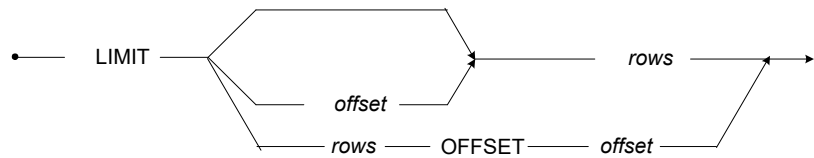
Figure 3-140 LIMIT syntax
