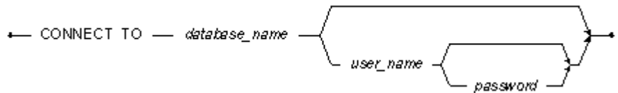
Figure 6-1 CONNECT syntax
