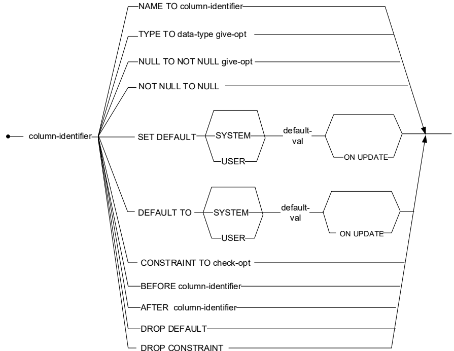
Figure 3-21 ATTRIBUTE-MODIFY-COLUMN-DEF syntax
