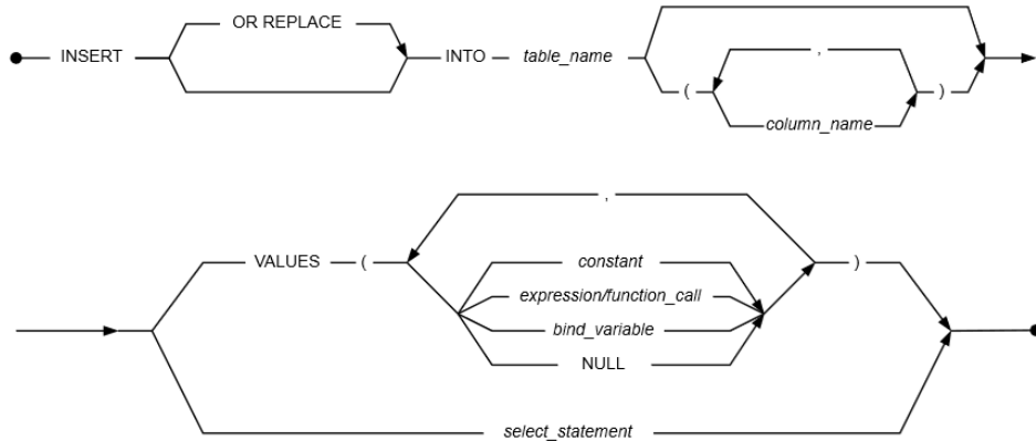
Figure 3-97 INSERT syntax
