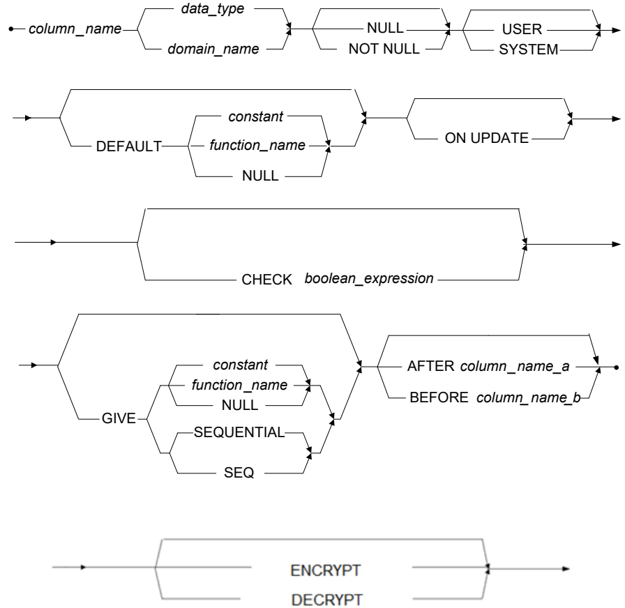
Figure 3-23 COLUMN_DEFINITIONS syntax
