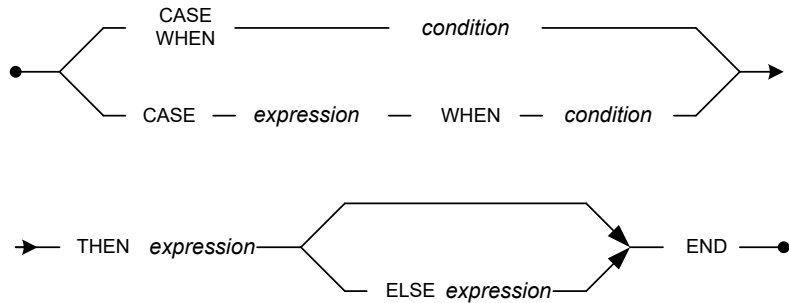
Figure 3-125 CASE Syntax
