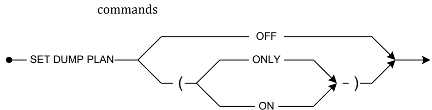
Figure 6-10 SET DUMP PLAN Syntax
