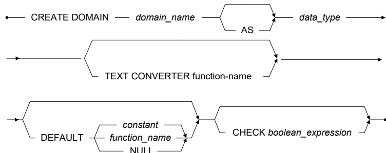
Figure 3-44 CREATE DOMAIN syntax
