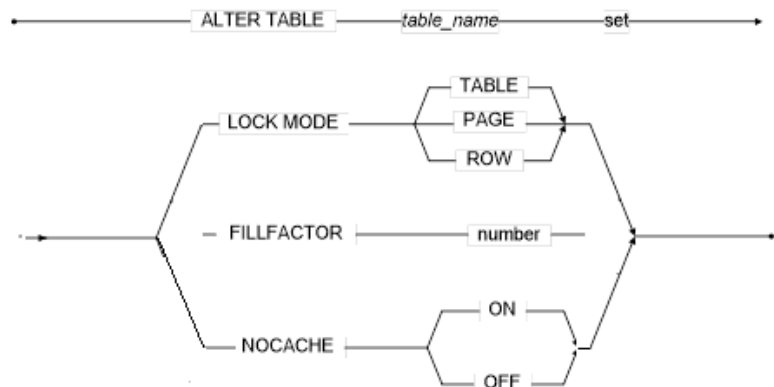
Figure 3-27 ALTER TABLE SET OPTIONS syntax
