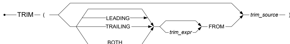
Figure 4-141 TRIM function syntax
