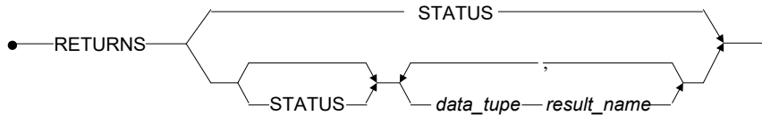
Figure 3-54 CREATE PROCEDURE: procedure_return_result syntax
