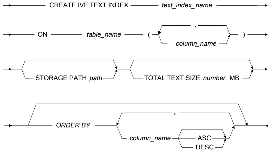
Figure 3-68 CREATE IVF TEXT INDEX syntax
