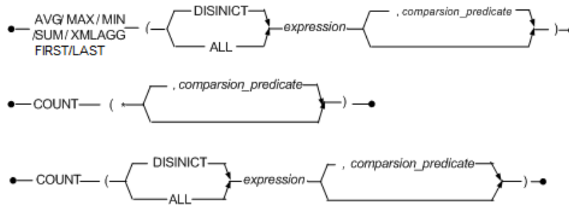
Figure 3-142 AGGREGATE FUNCTION syntax
