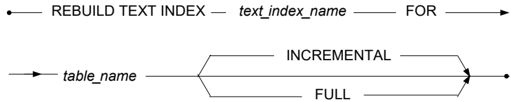
Figure 3-104 REBUILD TEXT INDEX syntax
