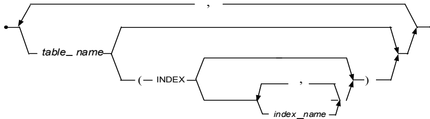
Figure 3-162 UPDATE STATISTICS Object List syntax
