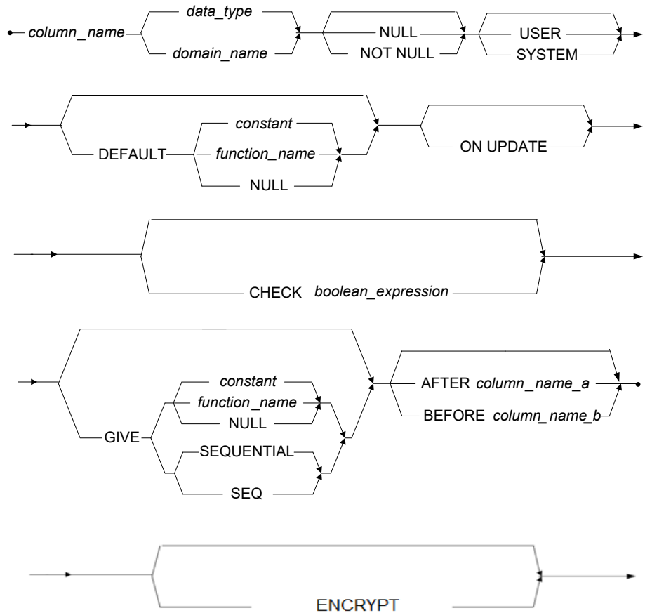
Figure 3-13 COLUMN DEFINITION syntax
