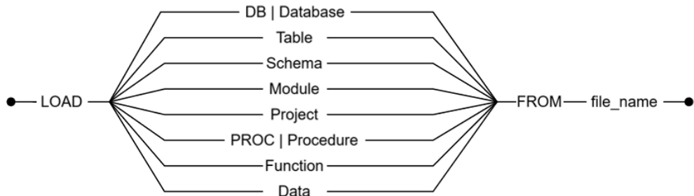
Figure 6-9 LOAD syntax
