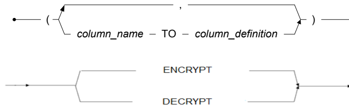
Figure 3-22 FULL-ATTRIBUTES-MODIFY-COLUMN-DEF syntax
