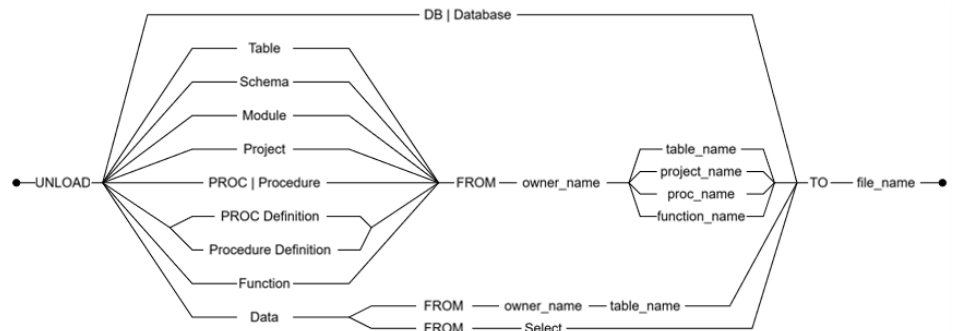
Figure 6-13 UNLOAD syntax
