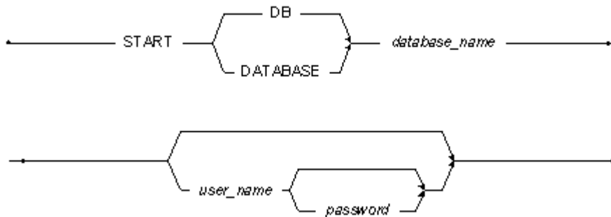
Figure 6-11 START DATABASE syntax
