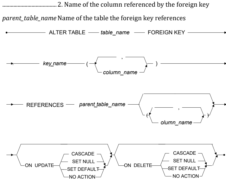
Figure 3-19 ALTER TABLE FOREIGN KEY syntax
