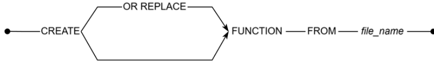
Figure 3-47 CREATE FUNCTION from file syntax
