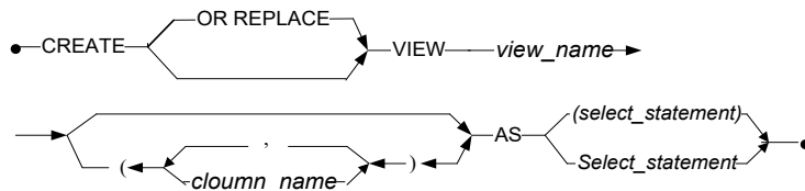
Figure 3-72 CREATE VIEW syntax
