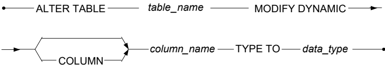
Figure 3-24 ALTER TABLE MODIFY DYNAMIC COLUMN syntax
