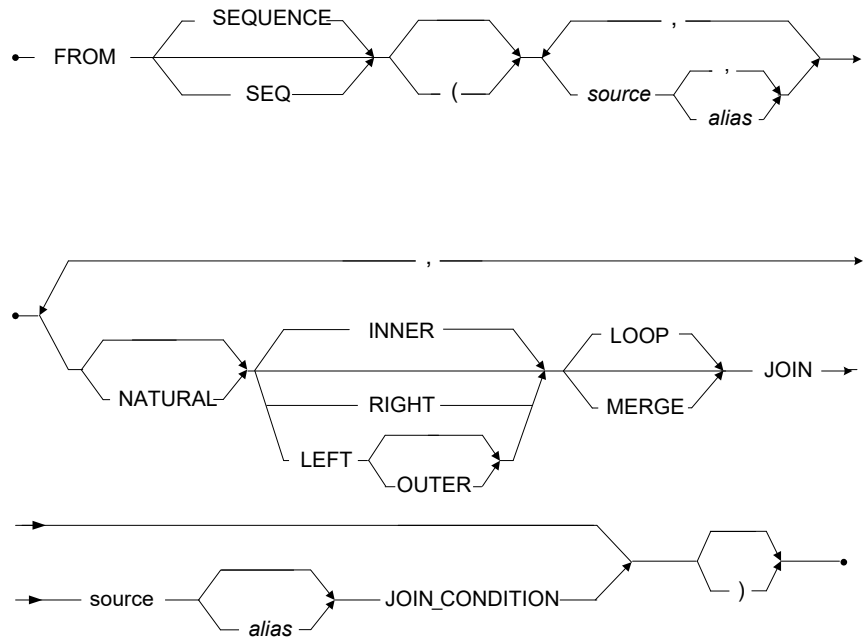
Figure 3-129 ANSI Join syntax
