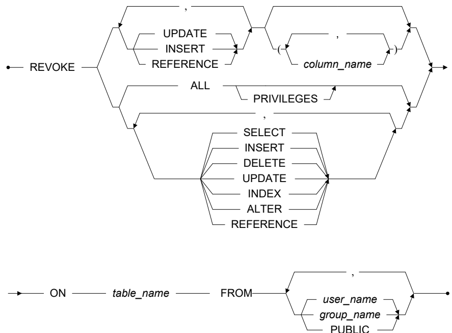
Figure 3-110 REVOKE (Object Privileges) syntax
