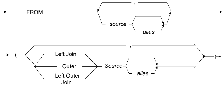
Figure 3-131 DBMaker Outer-Join Syntax
