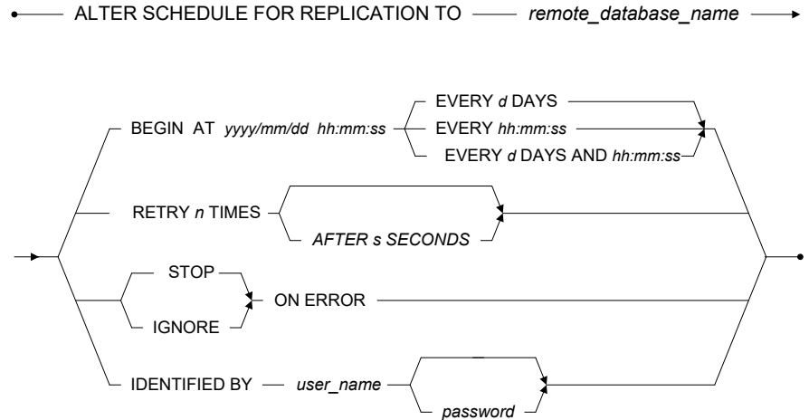
Figure 3-11 ALTER SCHEDULE syntax
