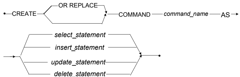
Figure 3-42 CREATE COMMAND syntax
