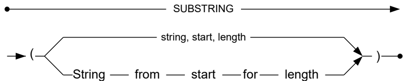
Figure 4-130 SUBSTRING syntax
