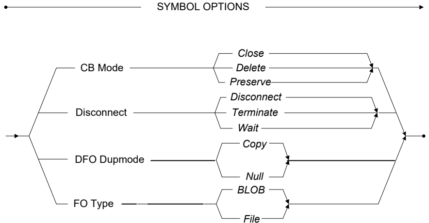
Figure 3-150 Symbol Options
